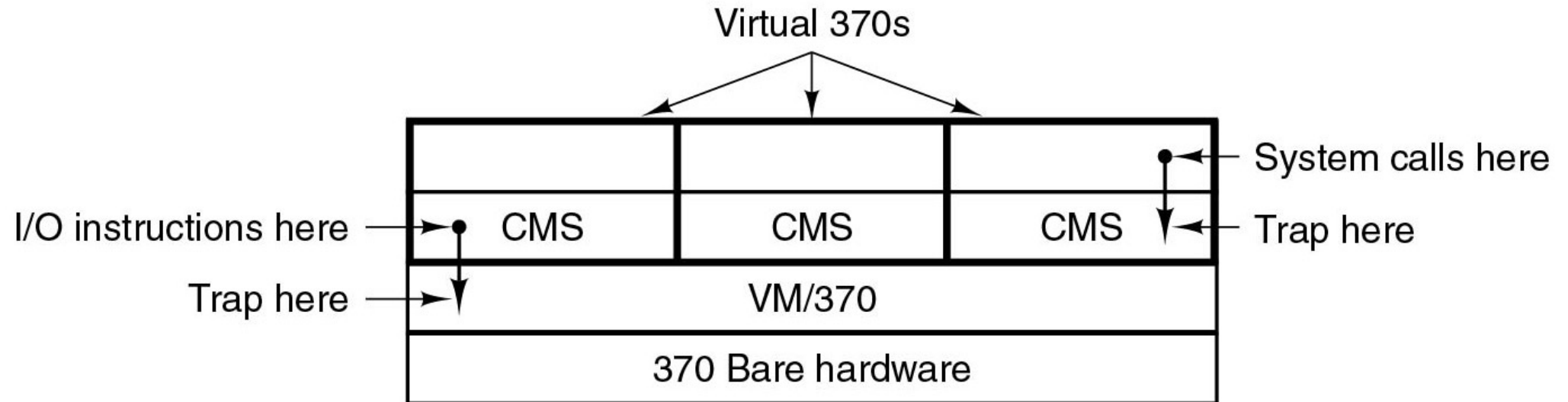
The structure of VM/370 with Conversational Monitor System (CMS)
